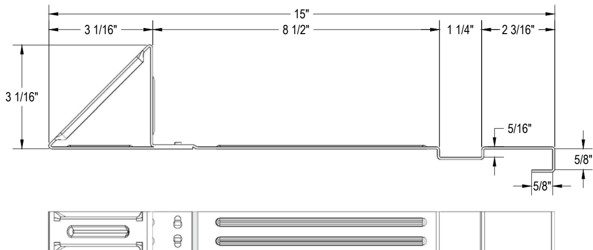
BRACKET DIMENSIONS (DO NOT SCALE)
