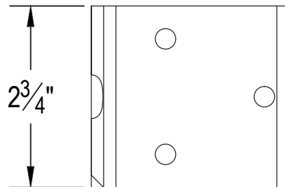
BRACKET DIMENSIONS
